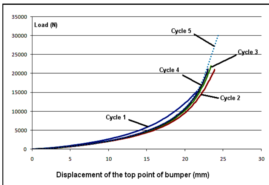
Fig. 11. Load - displacement curves of the bumper corresponding to the first 5 loading cycles at its top point
